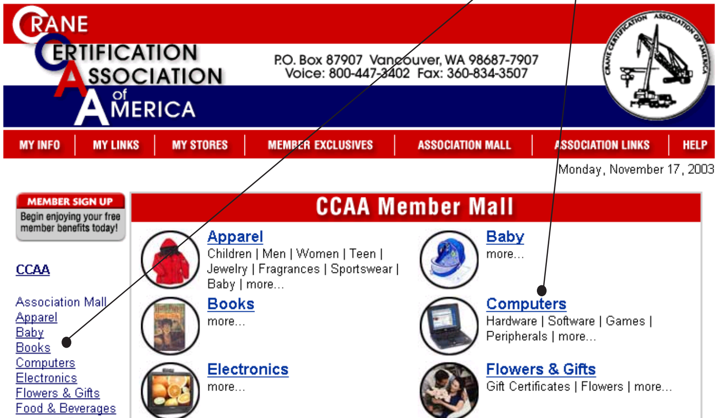
Figure 4 Member Mall
