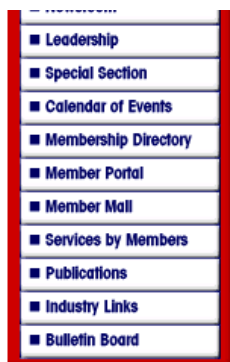
Figure 3 Left Navigation
